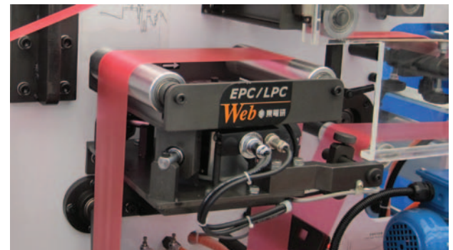
Center Pivot Guider C-200 is used on a Bag Making Machine
